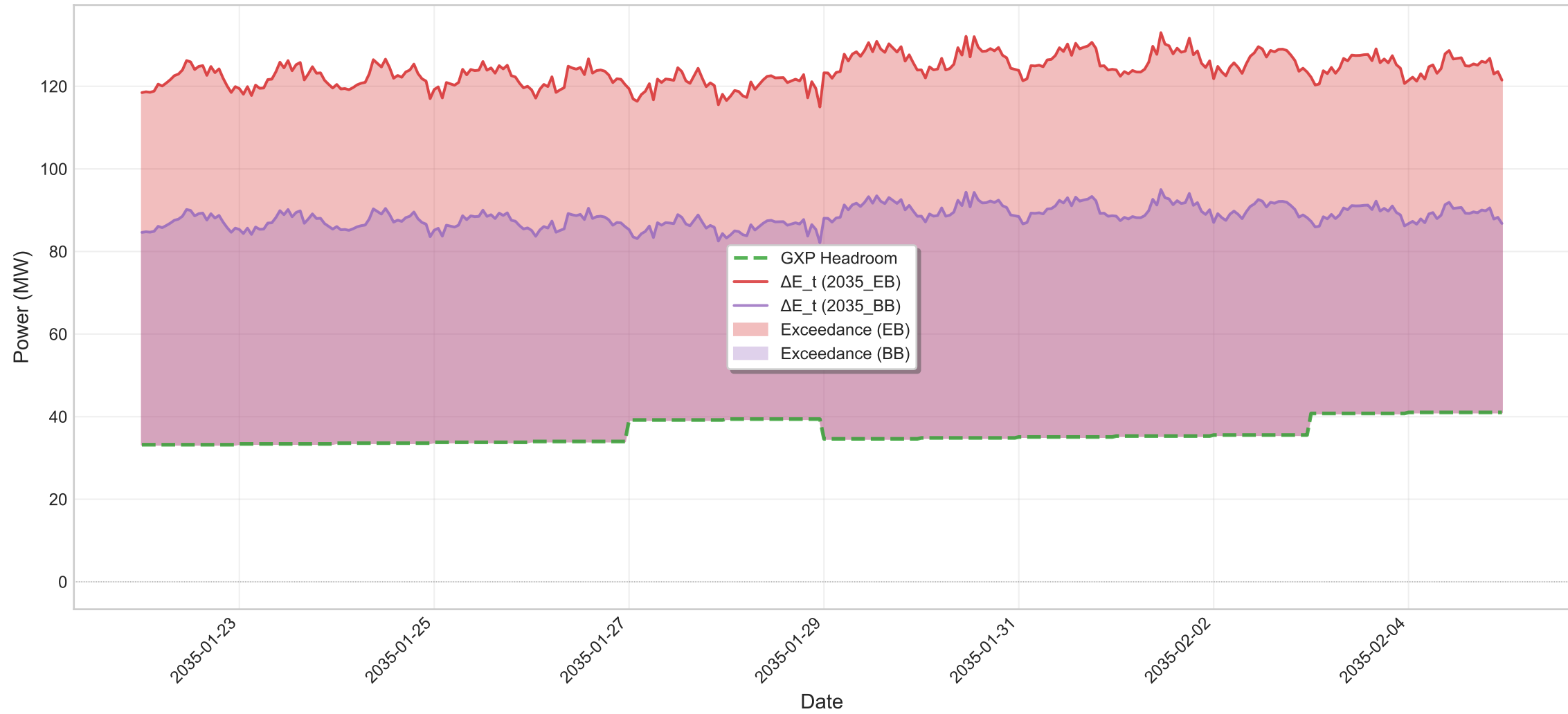
Incremental Electricity vs Headroom: 2035_EB vs 2035_BB Stress Window: 2035-01-22 to 2035-02-04
